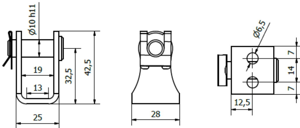
Dimensions mounting bracket i/con35: Rear
