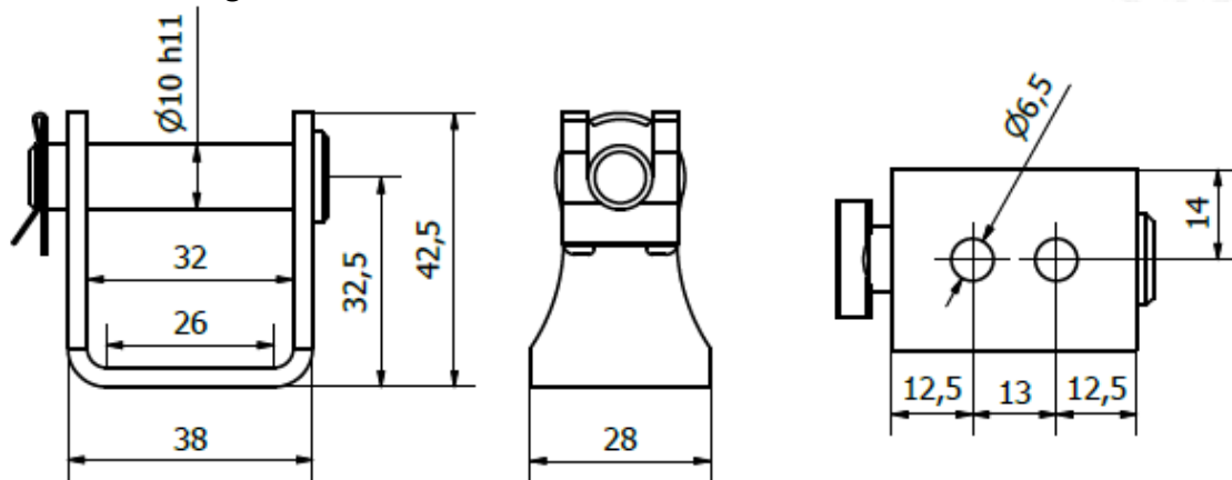
Dimensions mounting bracket i/con35: Rear
